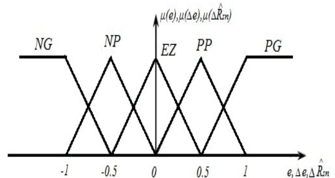
Fig. 4 Membership functions of inputs and output of fuzzy estimator
