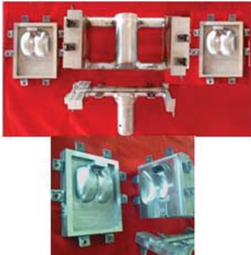
Fig. 3 The fabricated Pelton bucket mould components
