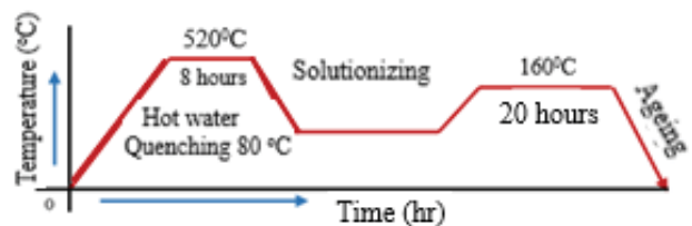
Fig. 7 Schematic of T6 Heat Treatment of A356-10%SiC composite profile
