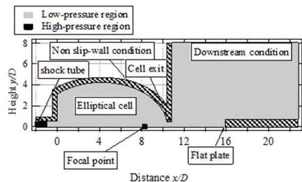
Fig. 1 Flow field for computation and boundary conditions
