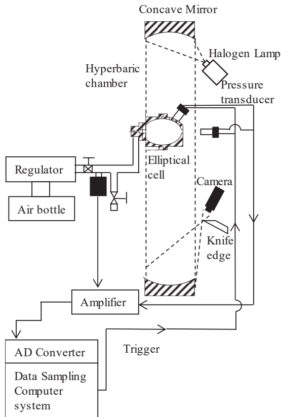
Fig. 2 Experimental apparatus
