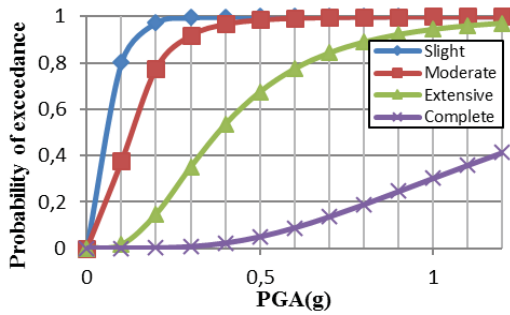
Fig. 7 Fragility Curve for Second Model; X-dir
