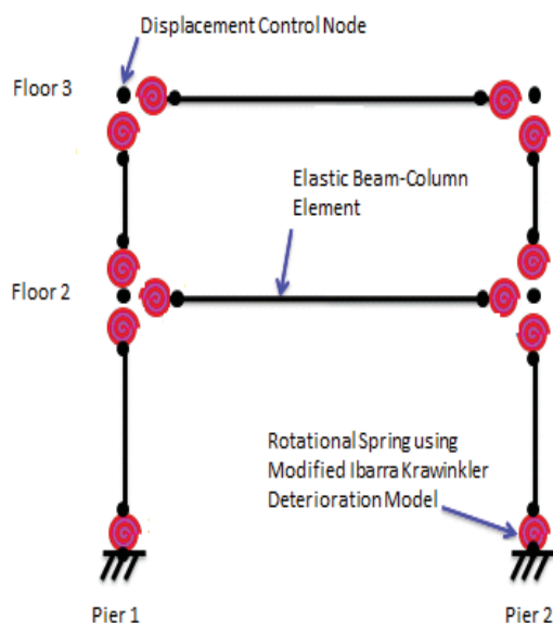
Fig. 5 Final proposed model
