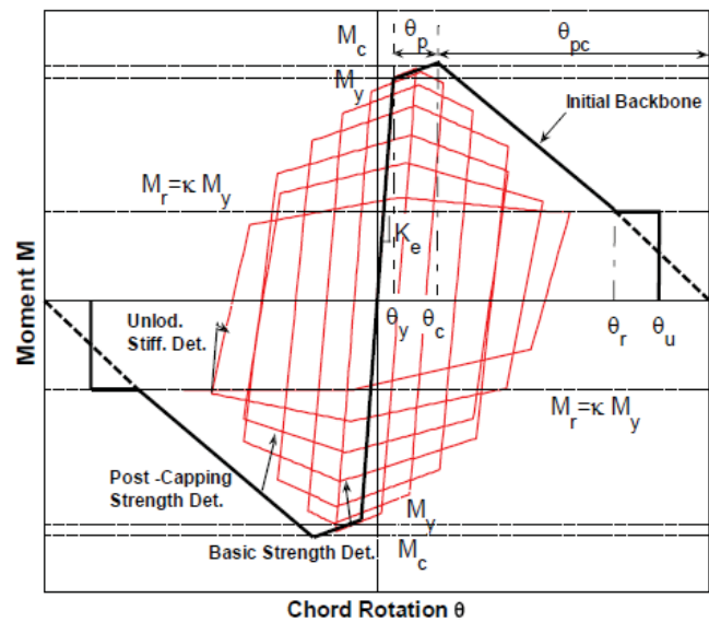
Fig. 4 Modified Ibarra Krawinkler Deterioration Model
