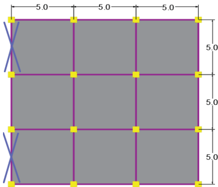
Fig. 2 Typical plan of 2 nd model
