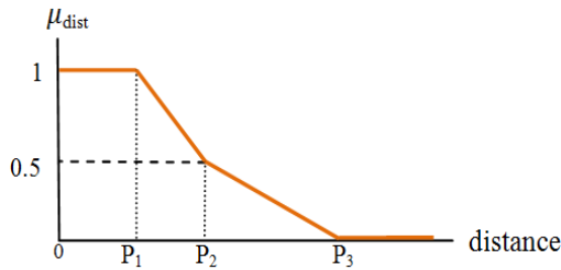
Fig. 1 Distance regions generated by piecewise linear function
