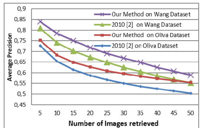
Fig. 6 Average precision at N (AP@N)
