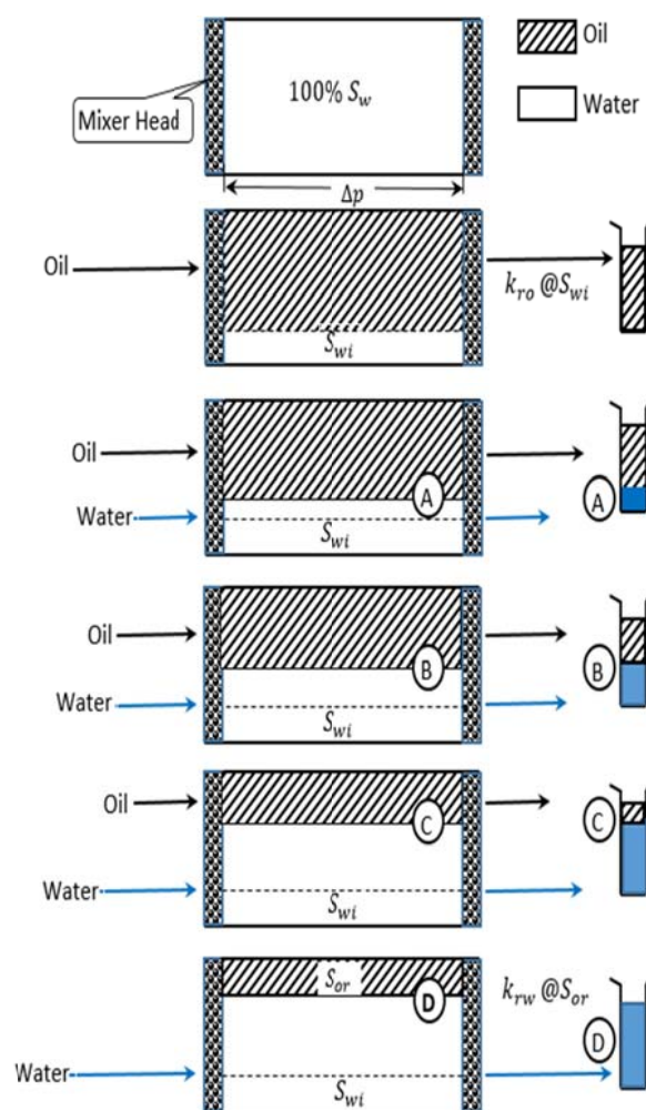
Fig. 1 Oil and water flow under various saturation [2], [3]
