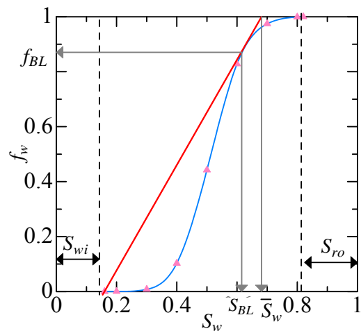
Fig. 5 Fractional flow
