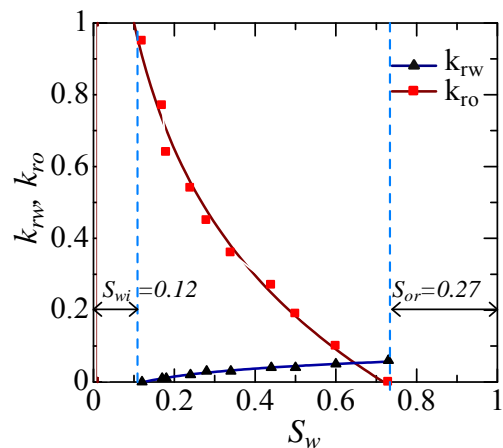
Fig. 2 Relative permeability curve of heavy oil
