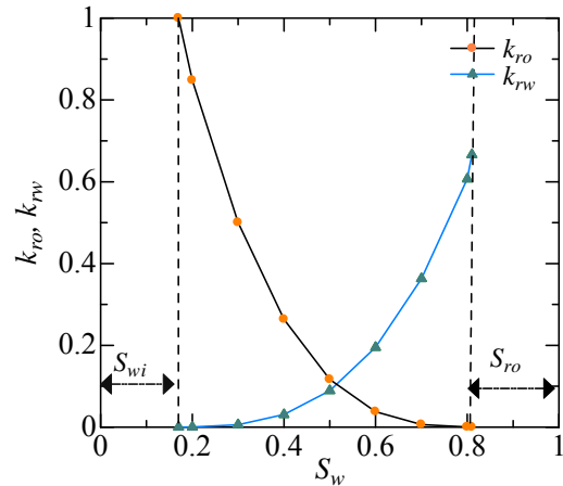
Fig. 4 Relative permeability curve of Light oil
