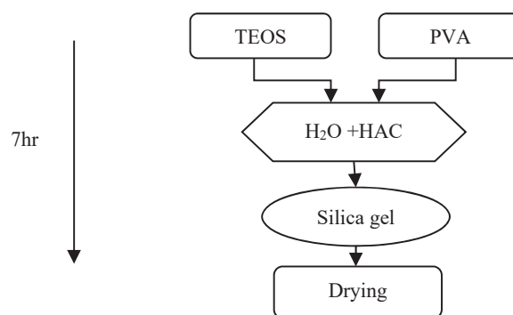
Fig. 1 Synthesis diagram
