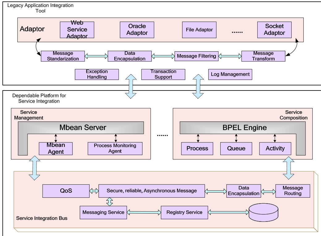
Fig. 1 The Architecture of SDIE
