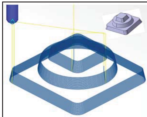
Fig. 6 Toolpath trajectory
