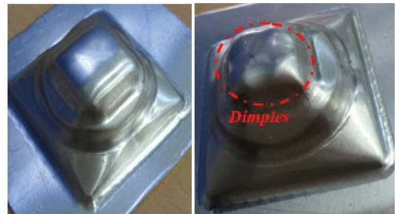
Fig. 7 Influence of the elastomeric interpolator
