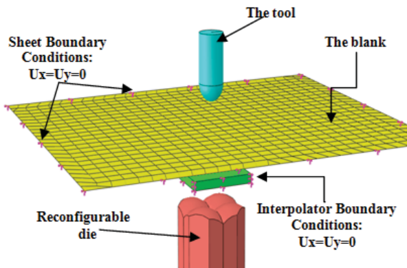
Fig. 5 Numerical model of the MPIF process
