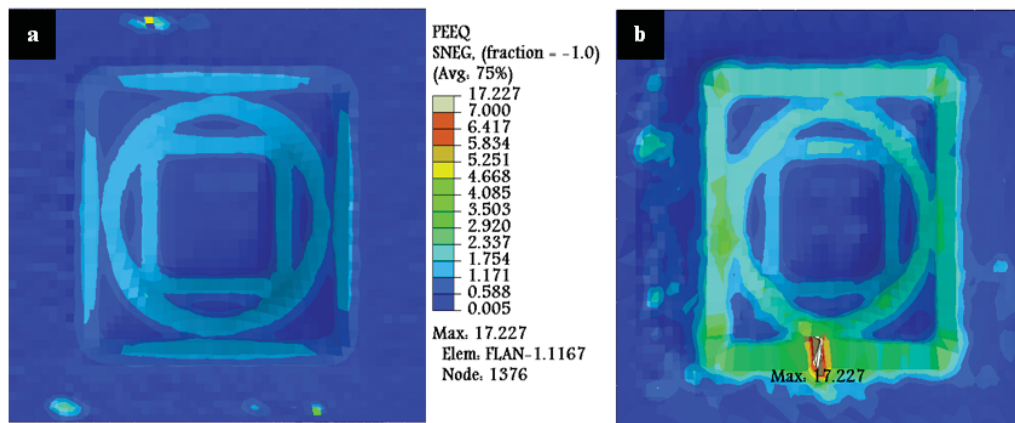
Fig. 10 Equivalent plastic strain distribution PEEQ (a) with an interpolator (b) without an interpolator
