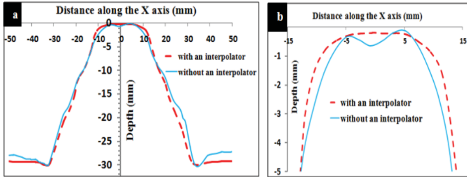
Fig. 8 Influence of the elastomeric interpolator
