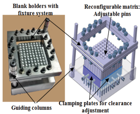
Fig. 2 Experimental set up of the MPIF process
