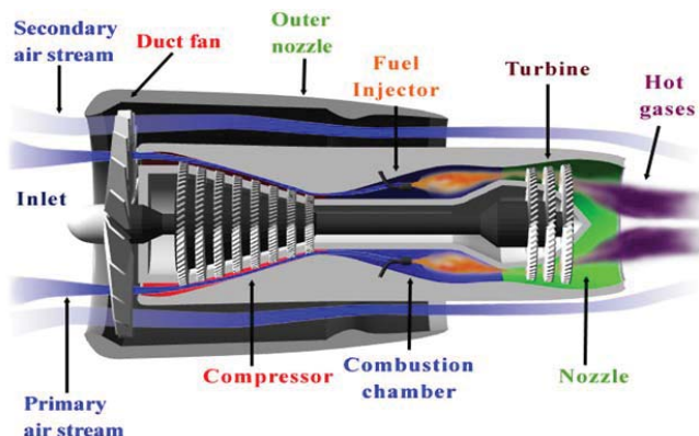
Fig. 1 Turbofan engine [11]
