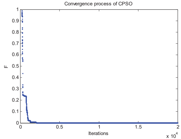
Fig. 4 Convergence process of CPSO
