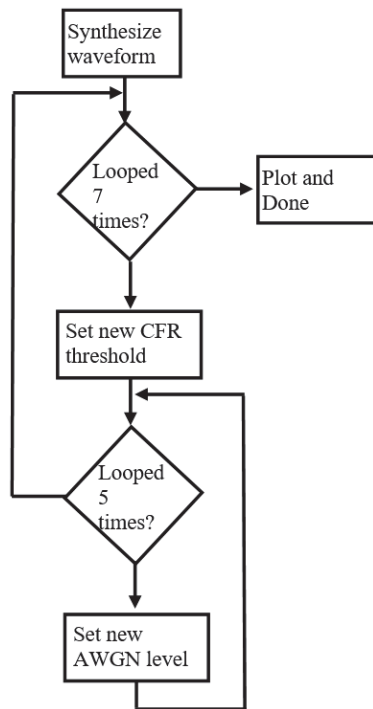
Fig. 1 Flow chart of the simulation algorithm
