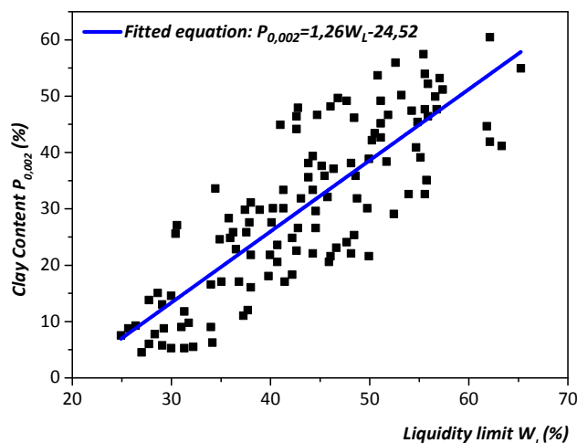
Fig. 4 Clay content as function of liquidity limit.
