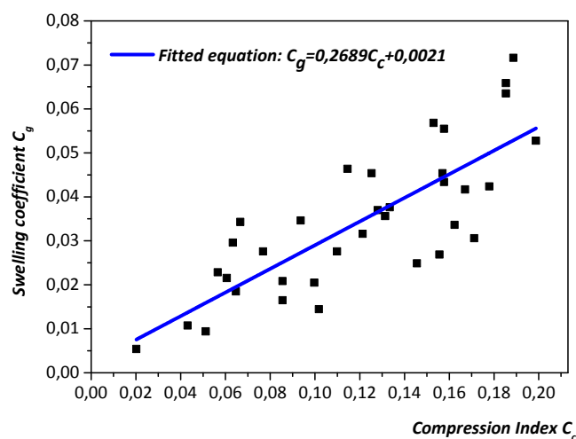
Fig. 6 Swelling coefficient as function of compression index
