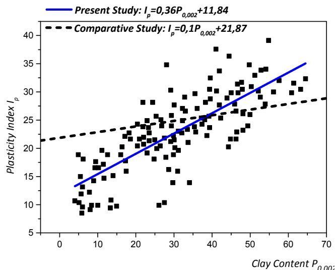
Fig. 5 Plasticity index as function of clay content
