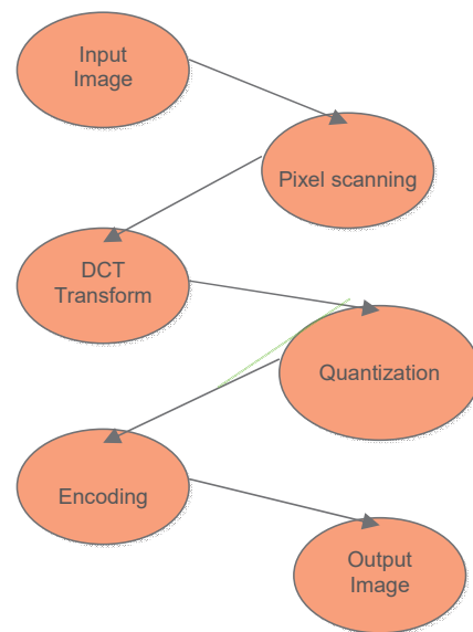
Fig. 2 JPEG Compression
