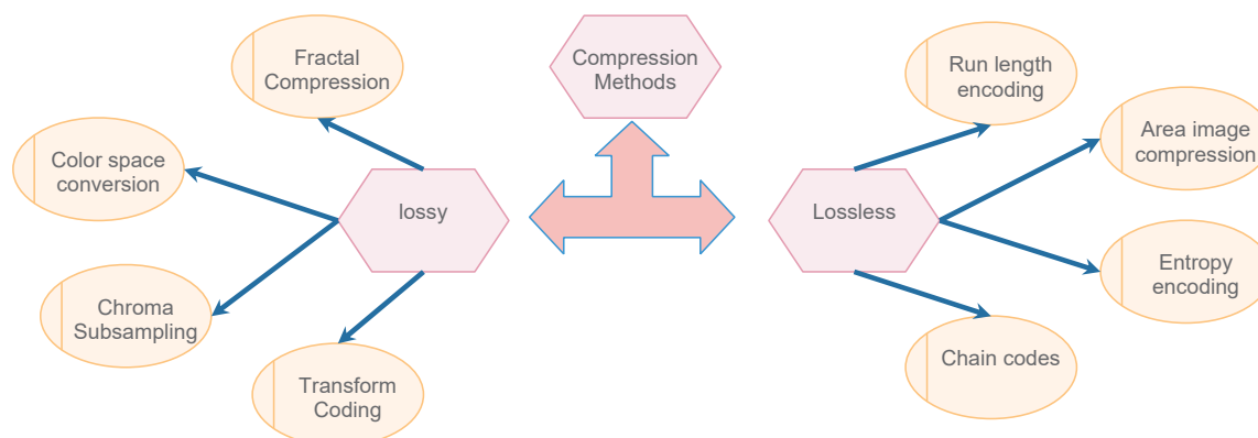
Fig. 1 Compression Methods
