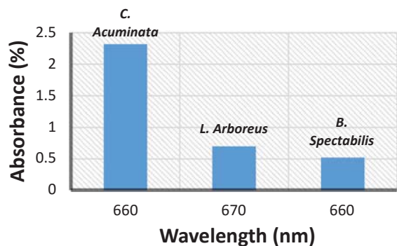
Fig. 3 Comparison of Absorbance against Wavelength for C. acuminata , L. arboreus and B. spectabilis
