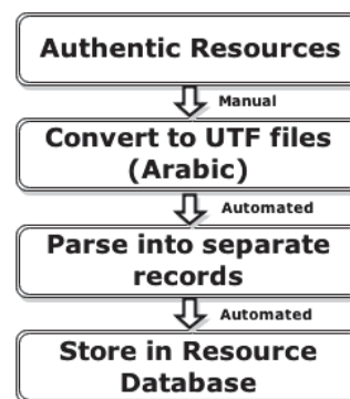
Fig. 1 Phase I - Raw data files to Resource database
