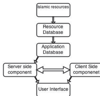
Fig. 3 Application architecture
