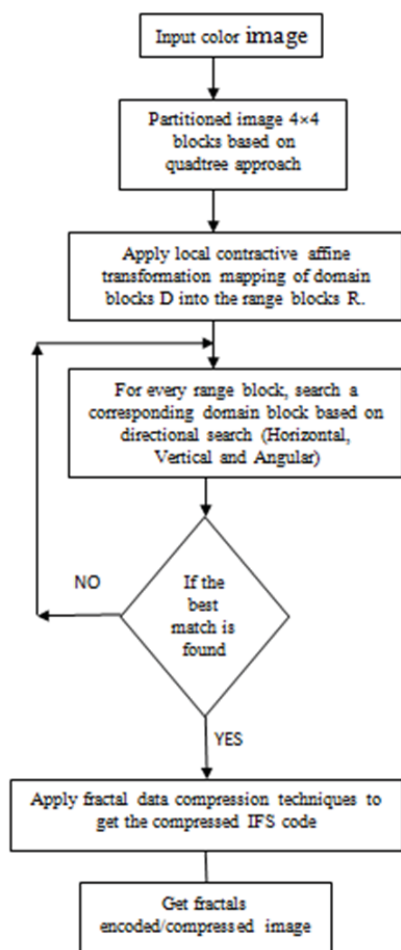
Fig. 1 The overall fractal encoding process
