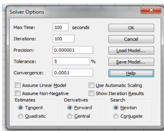
Fig. 2 Window of solver options
