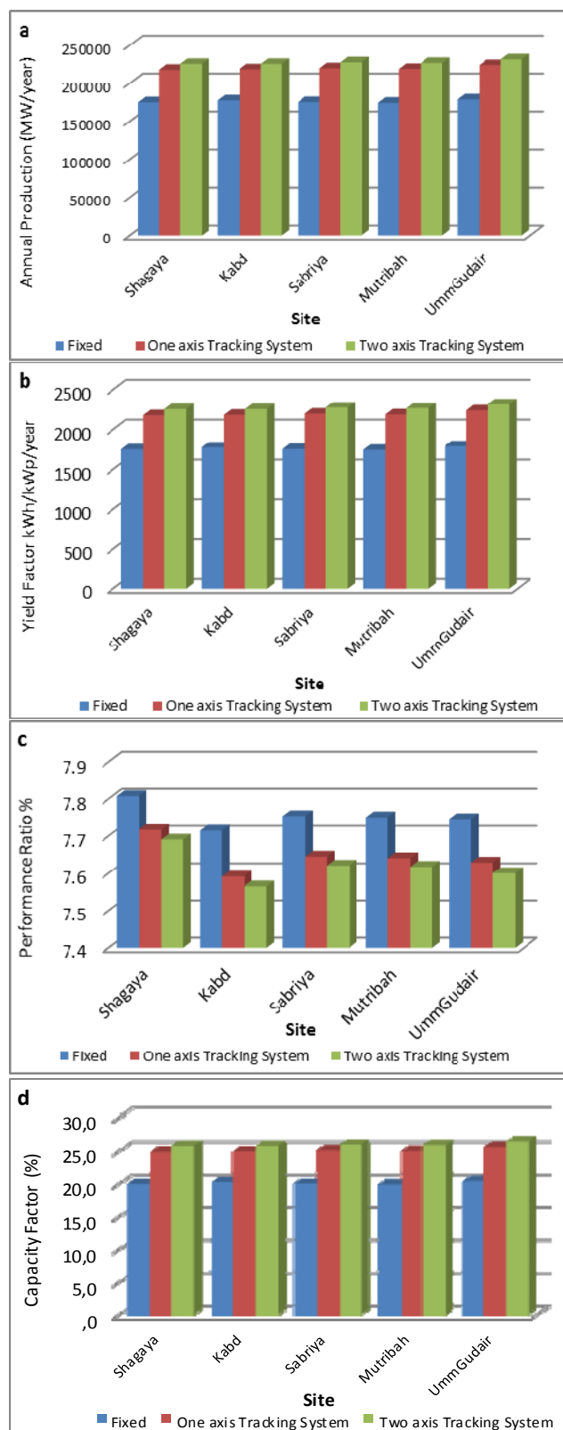
Fig. 3 Performance parameters for the selected sites: (a) Annual Production, (b) Yield Factor, (c) PR, (d) CF
