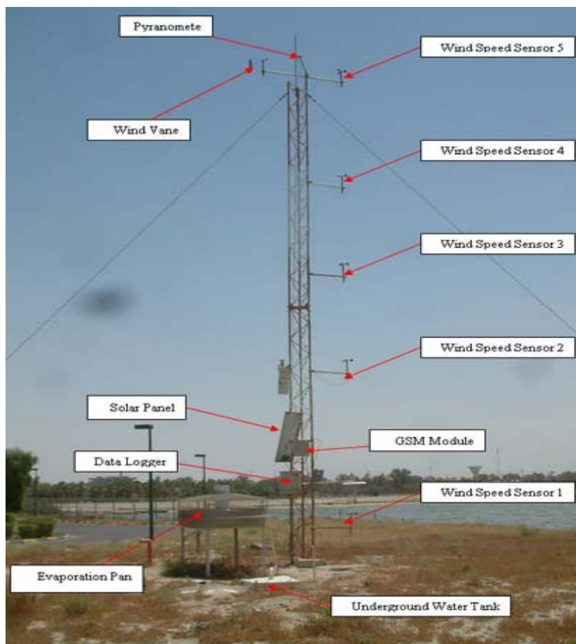
Fig. 2 A typical meteorological station [9]
