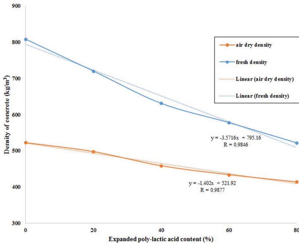
Fig. 1 The relationship between density and PLA ratio
