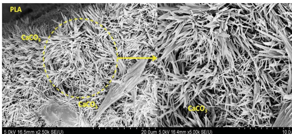
Fig. 5 Interfacial transition zone (ITZ) of vermiculite concrete with 80% PLA
