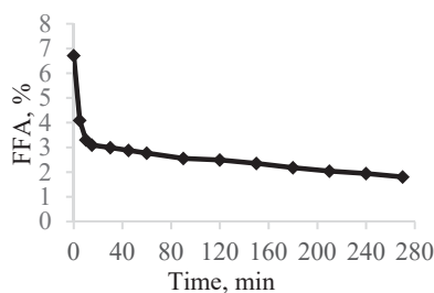
Fig. 1 Esterification of CPO
