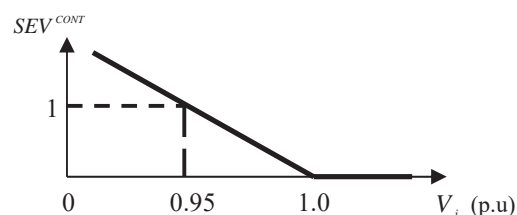
Fig. 1 Continuous severity function for low voltage
