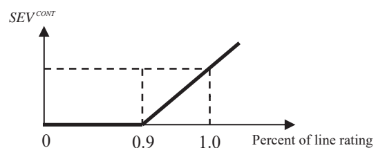
Fig. 2 Continuous severity function for line overload
