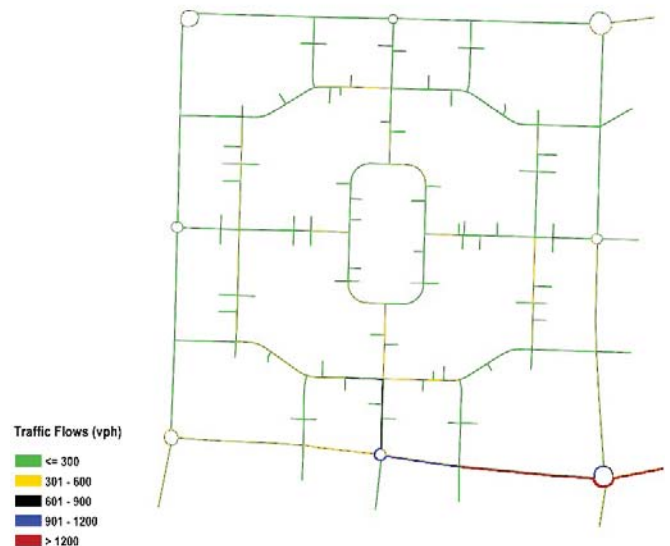
Fig. 16 2030 AM Peak Traffic Flows – Rectilinear Residential Area
