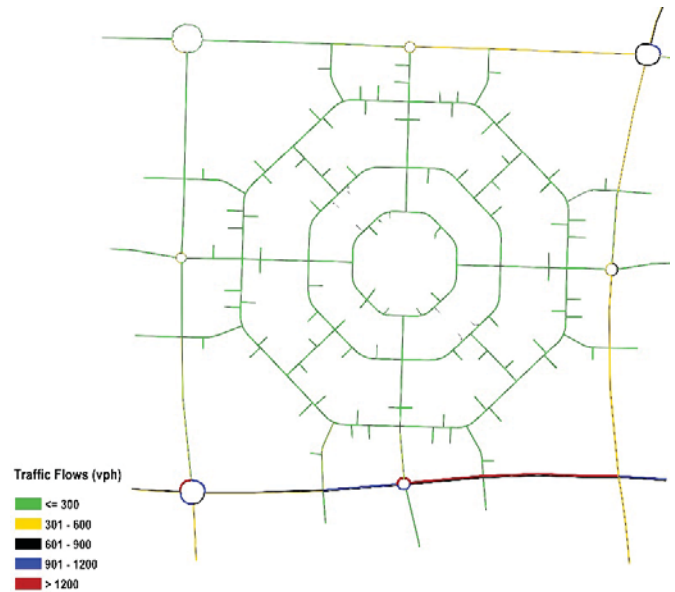
Fig. 15 2030 PM Peak Traffic Flows – Octagonal Residential Area
