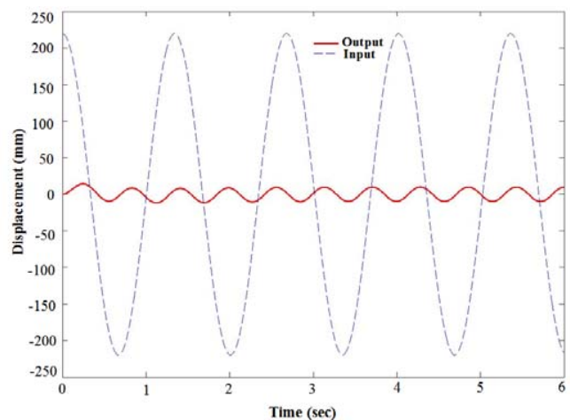
Fig. 7 Displacement response with respect to time history
