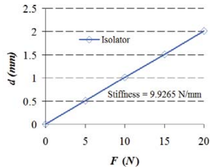
Fig. 17 Force-to-displacement curve of the isolator
