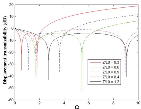
Fig. 9 Effect of input displacement on transmissibility
