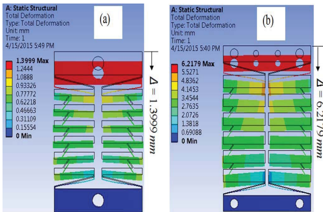
Fig. 15 Deformation of: (a) horizontal spring, (b) vertical spring
