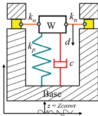
Fig. 6 Schematic diagram of dynamic model
