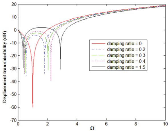
Fig. 8 Effect of damping ratio on displacement transmissibility
