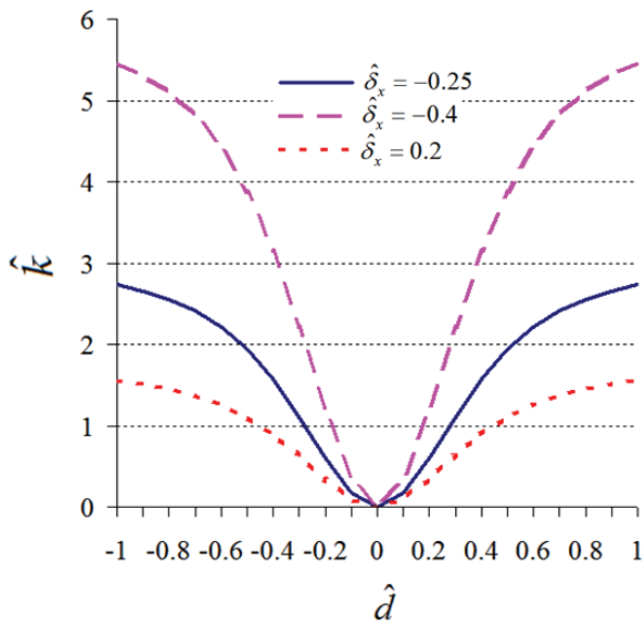
Fig. 5 Stiffness curves for different \hat{\delta}_x
