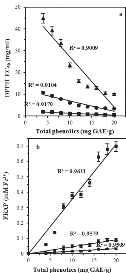
Fig. 2 Correlation between the antioxidant activity of peel (■), seed (●) and juice (▲) extract determined by the DPPH (a) and FRAP (b) method. Data are mean (n = 3) ± standard deviation (n = 3), (p < 0.05)
