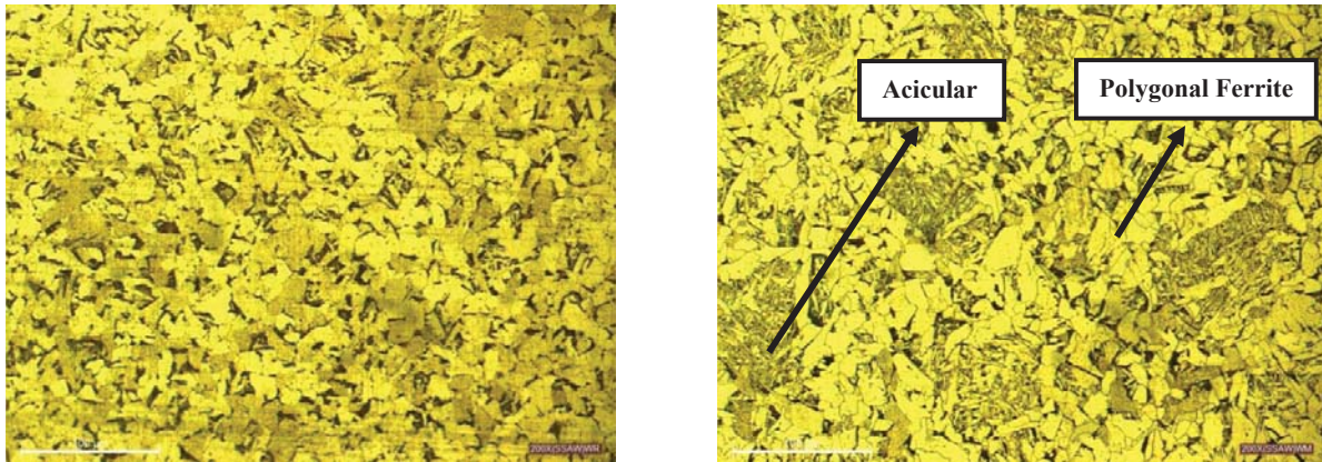
Fig. 7 (a) Microstructure of WZ (Root portion) at 200X
