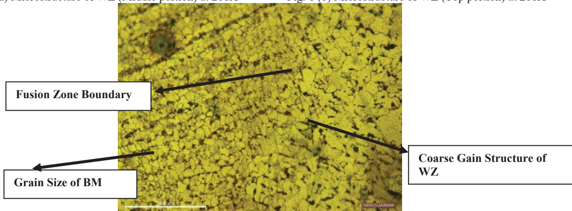
Fig. 6 (c) Microstructure of HAZ at 500X
