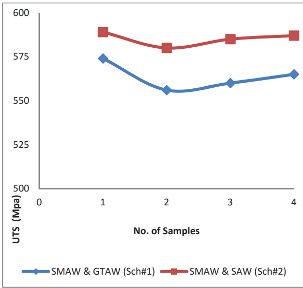
Fig. 1 UTS Comparison of Schemes 1 & 2
