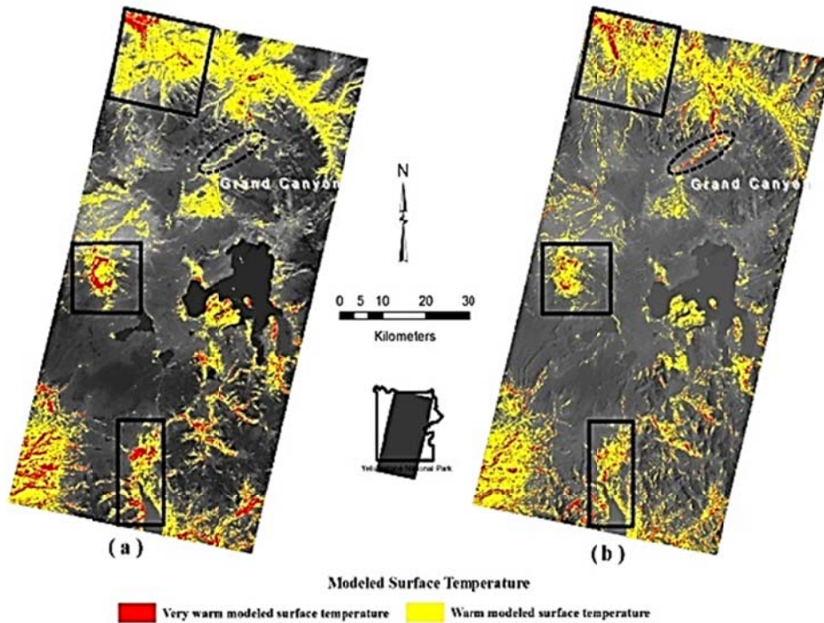
Fig. 6 (a) Thermal anomalies derived from ASTER daytime surface temperature, and (b) Thermal anomalies derived from the residual temperature (boxes show some areas where the topographic and solar effects were eliminated or significantly reduced)
