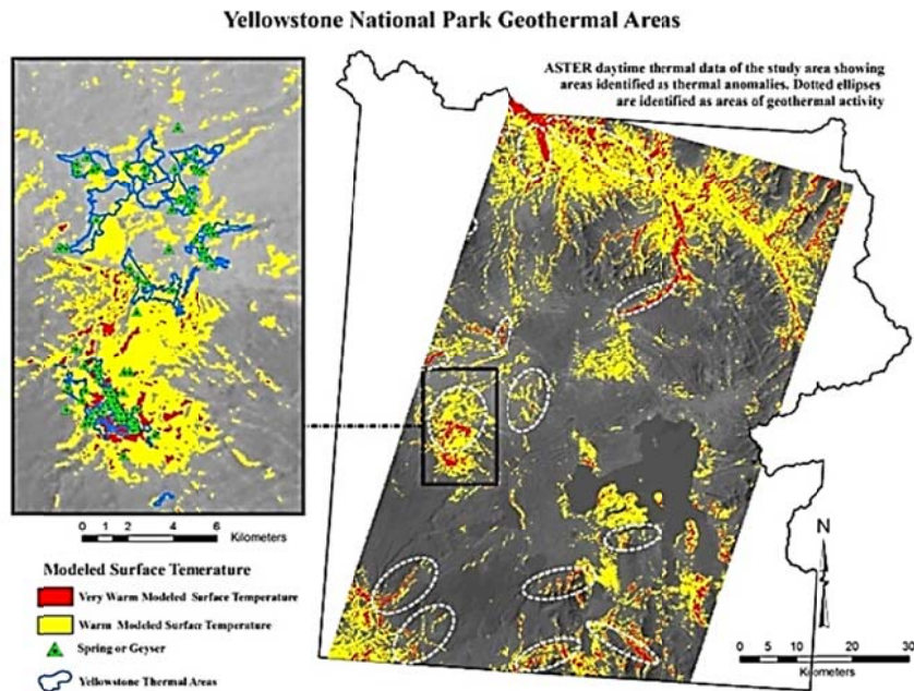
Fig. 8 ASTER daytime thermal data of the study area showing areas identified as thermal anomalies (dotted ellipses are identified as areas of geothermal activity (right). Lower and Midway thermal areas, springs and geysers superimposed on ASTER daytime thermal anomalies (left))
