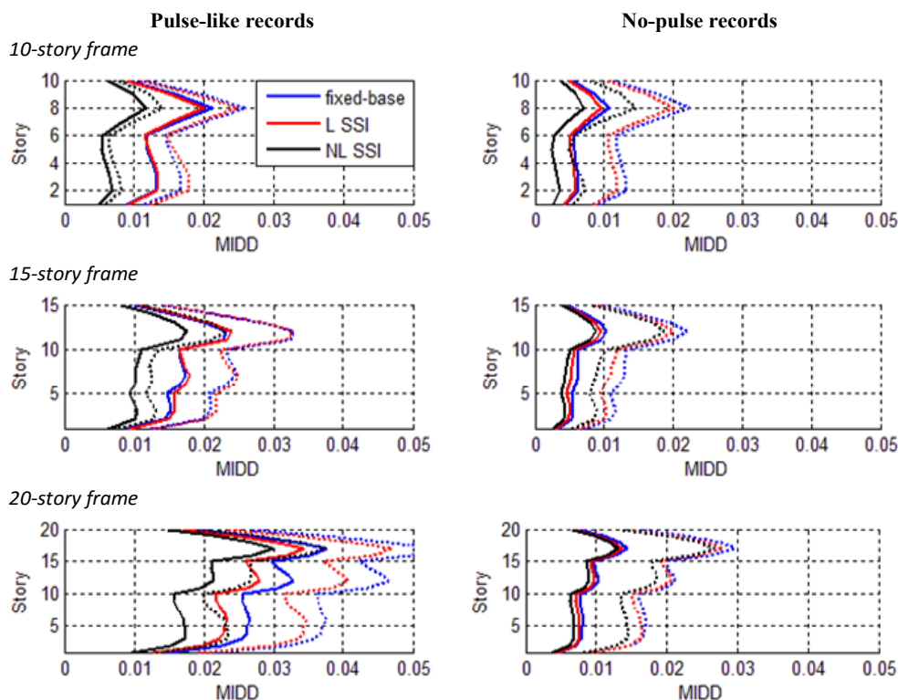
Fig. 6 MIDD distribution of “non-ductile” frame at MCE level (Dash lines indicate mean+ \sigma )
