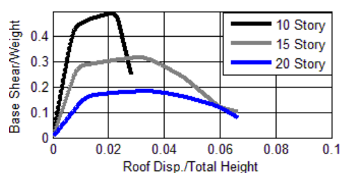
Fig. 1 Capacity curves of the designed steel frames using pushover analysis
