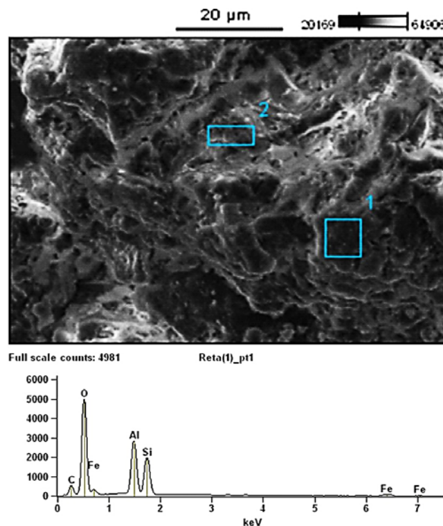
Fig. 4 SEM micrograph and EDS spectrum of WTR
