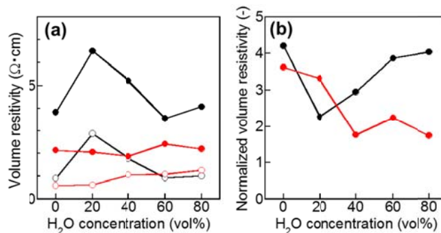
Fig. 4 Volume resistivities of various particle powders versus H 2 O concentration in surface-modification (a graph (a)). Open and closed circles: ITO particles for 0 and 10 days after surface-modification, respectively. A graph (b) shows normalized volume resistivities versus H 2 O concentration. The volume resistivities were normalized with that for 0 day. Black and red plots: ITO particles surface-modified with MPS and APMS, respectively
