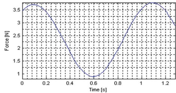
Fig. 15 One of the 54 sample records of the interaction force in Y direction which corresponds to the piezo pos. data sample shown in Fig. 6
