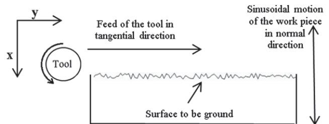
Fig. 3 Grinding Process
