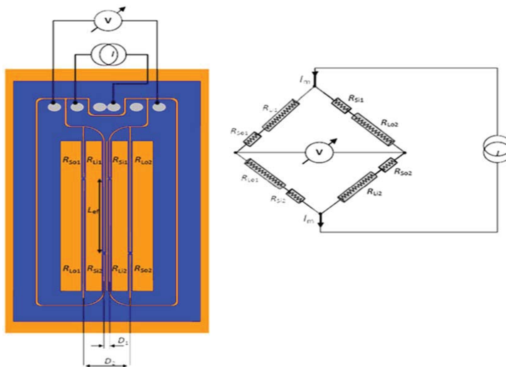
Fig. 1 THB6K sensor and equivalent electrical circuit diagram [24]
