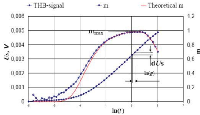
Fig. 2 Typical response of THB sensor [24]
