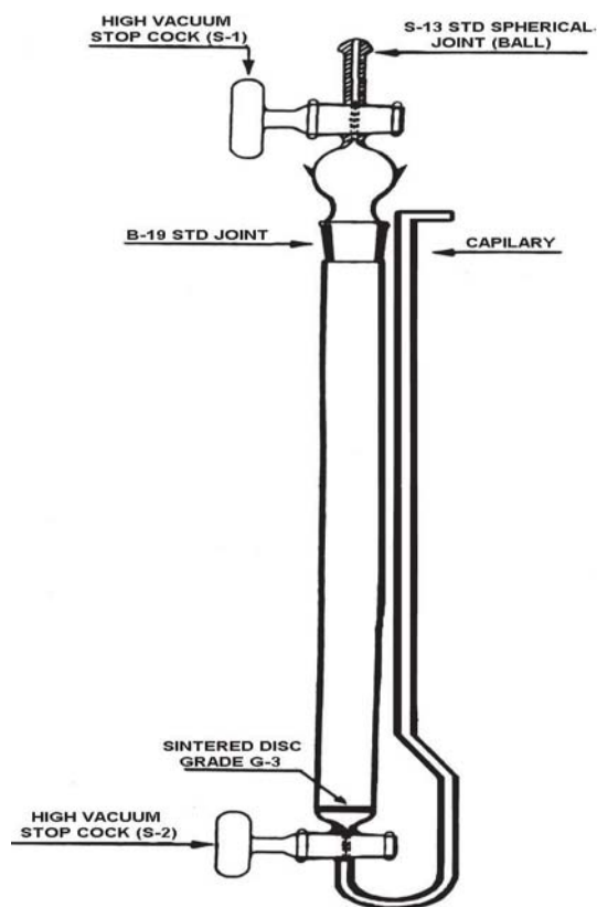
Fig. 2 Radon Bubbler
