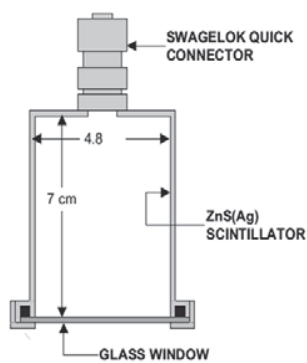
Fig. 3 Scintillation cell
