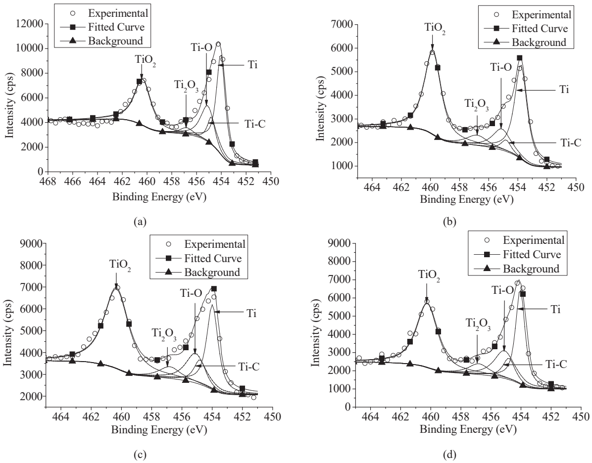
Fig. 7 Typical curve fitting conducted for Ti2p high resolution XPS spectra obtained from the Ti side of the joined samples after ion-milling to the depth of 480 nm: (a) sample 1; (b) sample 2; (c) sample 3; (d) sample 4
