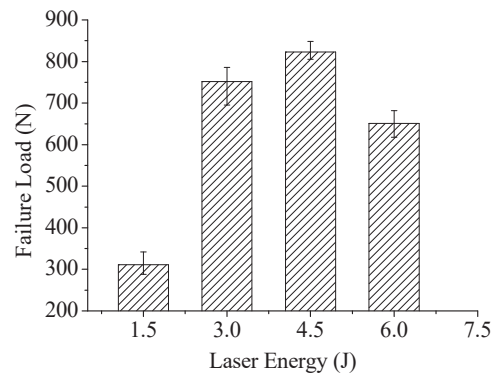
Fig. 10 The effects of laser energy on tensile failure load
