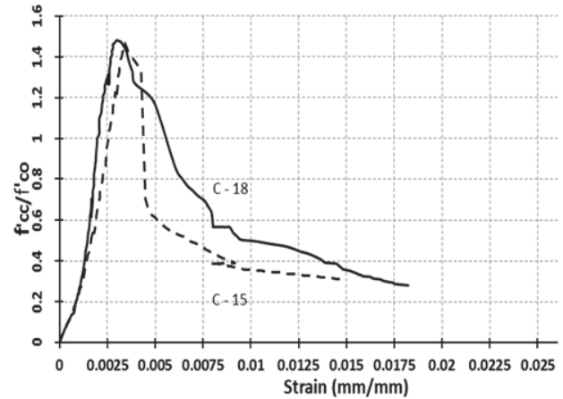
Fig. 5 Effect of concrete compressive strength
