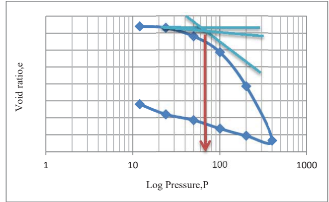
Fig. 3 Consolidation Curve (Fully Automatic Consolidated) Based on Pre-Consolidation a Typical e-log p Curve
