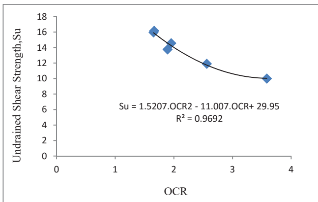
Fig. 5 Relationship between Su and OCR for Borehole (1)
