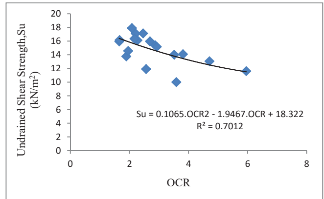
Fig. 6 Relationship between Su and OCR for Average of Three Boreholes
