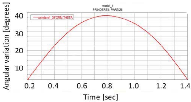
Fig. 11 Knee modular orthosis angular variation during a simulation
