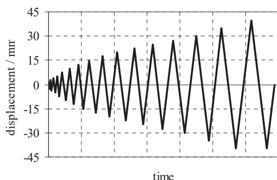
Fig. 16 Loading history
