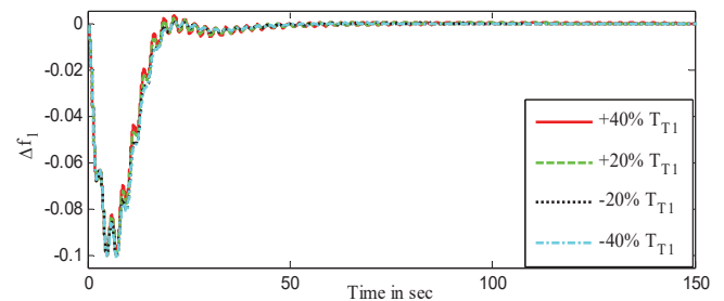
Fig. 18 Frequency deviation of area-1 for load change of 1% in area-2 with variation in T_{T1}
