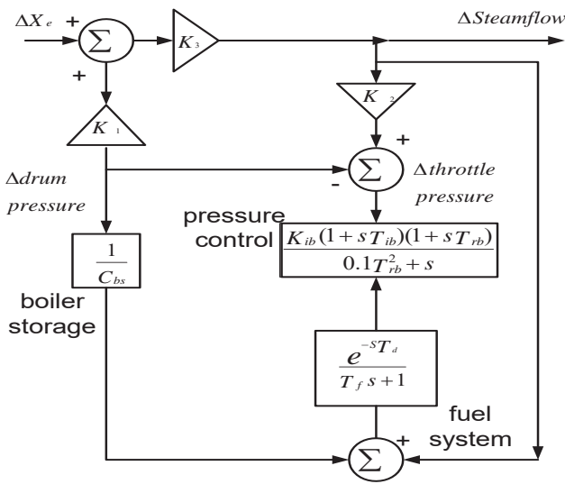
Fig. 3 Boiler dynamics
