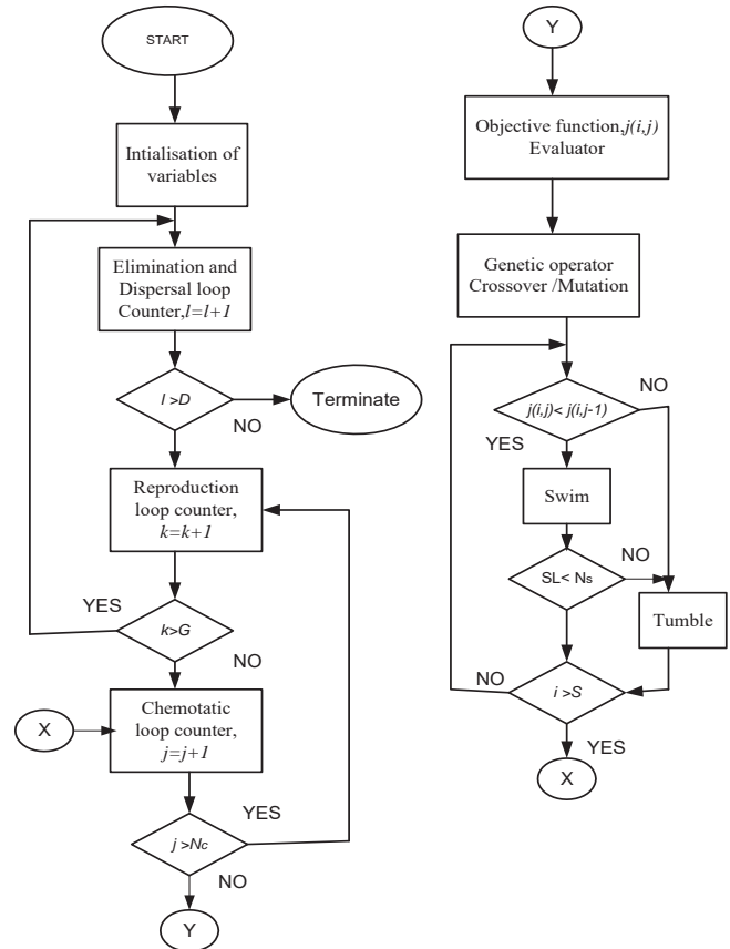
Fig. 5 Flow chart of BFOA
