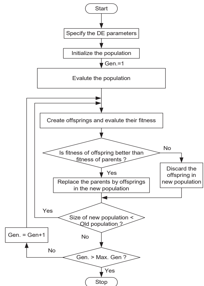
Fig. 6 Flow chart of DE
