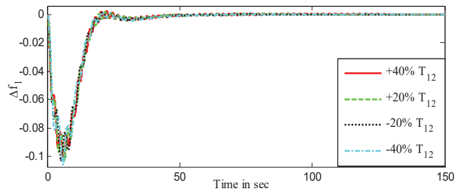
Fig. 19 Frequency deviation in area-1 for step load change of 1% in area-2 with variation in T_{12}
