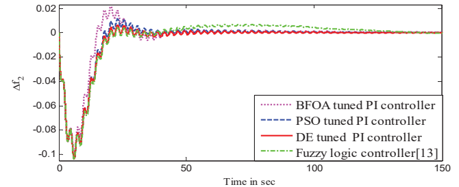
Fig. 10 Frequency deviation of area-2 for load change of 1% in area-2
