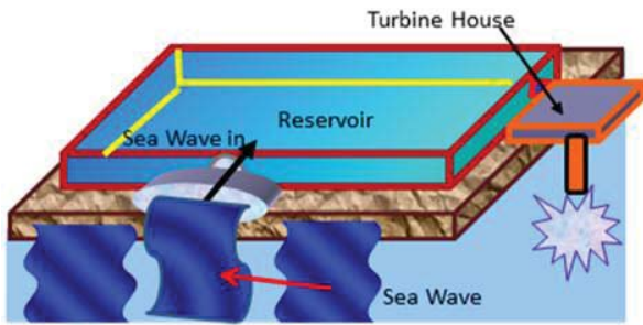
Fig. 2 Wave convergence energy reservoir device
