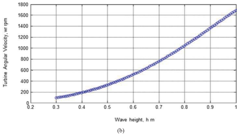
Fig. 13 Relation between the wave height and a- air velocity at the turbine entrance, and b- the turbine rotational velocity
