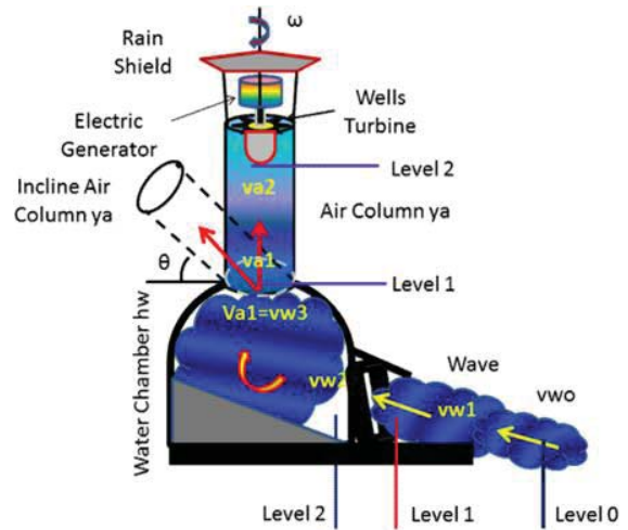
Fig. 4 General sketch for the present project
