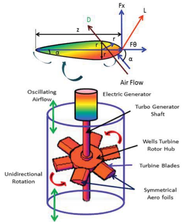
Fig. 5 Air velocity diagram on the turbine blades
