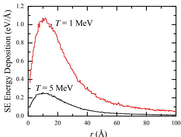
Fig. 3 Monte Carlo simulation of the radial energy deposited by secondary electrons produced by a 1 MeV and 5 MeV proton beam impinging on PMMA, as a function of the radial distance r from the ion impact. The energy is deposited in spherical shells of inner radius r and outer radius r + dr
