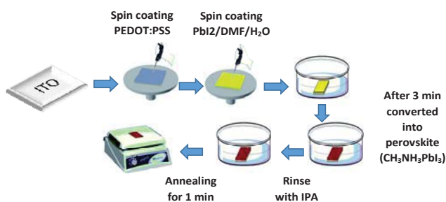
Fig. 1 Schematic illustration of the sequential deposition process
