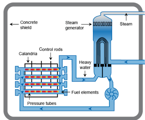
Fig. 4 CANDU Reactor [2]
