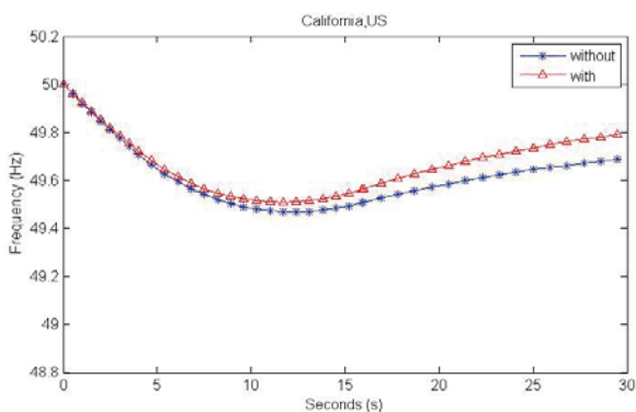
Fig. 6 Primary Frequency Response for California, US
