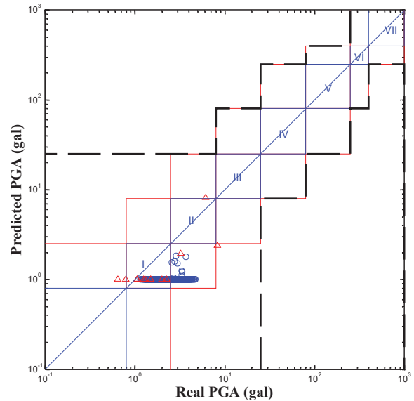
Fig. 11 Measured PGA and predicted PGA values using the SVM method when the seismometer was installed at a depth of 40 meters in the third stage with a smaller trigger threshold
