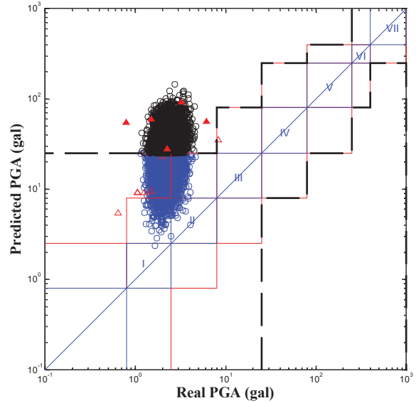
Fig. 10 Measured PGA and predicted PGA values using the TPA method when the seismometer was installed at a depth of 40 meters in the third stage with a smaller trigger threshold
