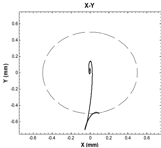
Fig. 9 Shaft trajectory obtained by implementing a simple non-hybrid linear control in dynamic mode
