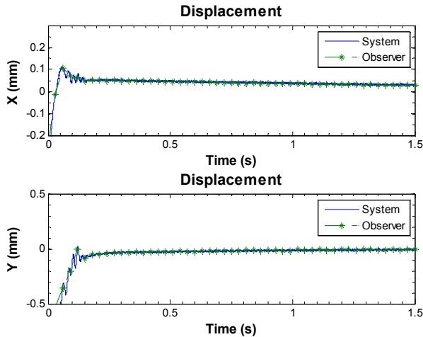
Fig. 20 Trajectory of shaft axis in experimental test for the non-hybrid linear method in the static mode
