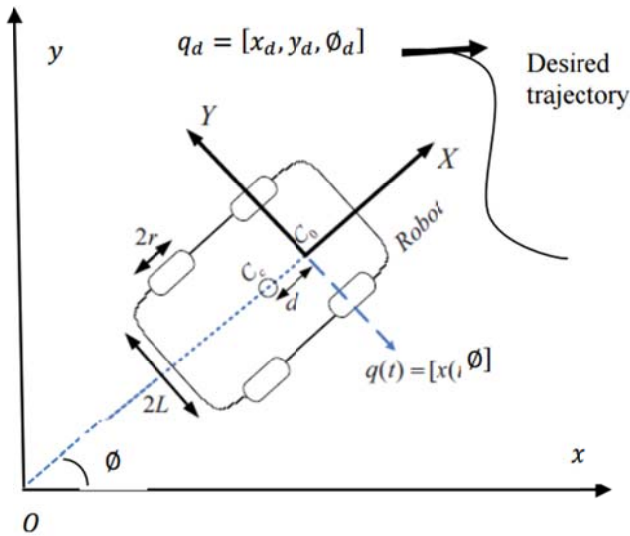
Fig. 1 Mobile robot
