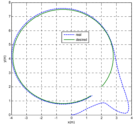
Fig. 9 Tracking trajectory in (X, Y) plan
