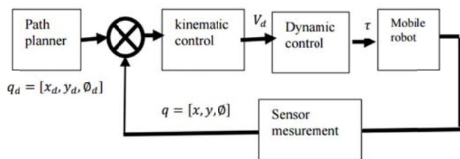
Fig. 2 Control design
