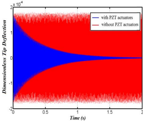
Fig. 4 Control of FG-CNTRC beam under follower force
