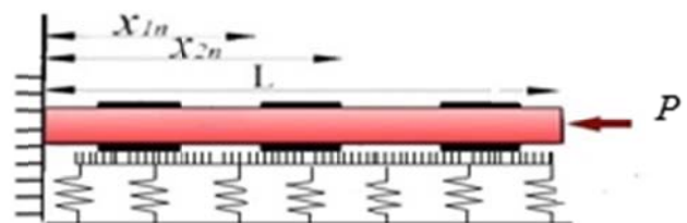
Fig. 1 FG-CNTRC beam resting on elastic foundation
