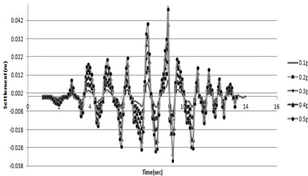
Fig. 3 Settlement and uplifting for unanchored tank in dense soil
