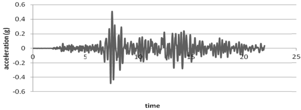
Fig. 2 Time history acceleration
