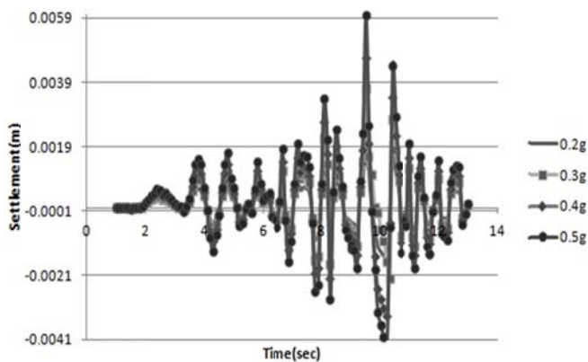
Fig. 8 Settlement and uplifting for anchored tank in loose soil
