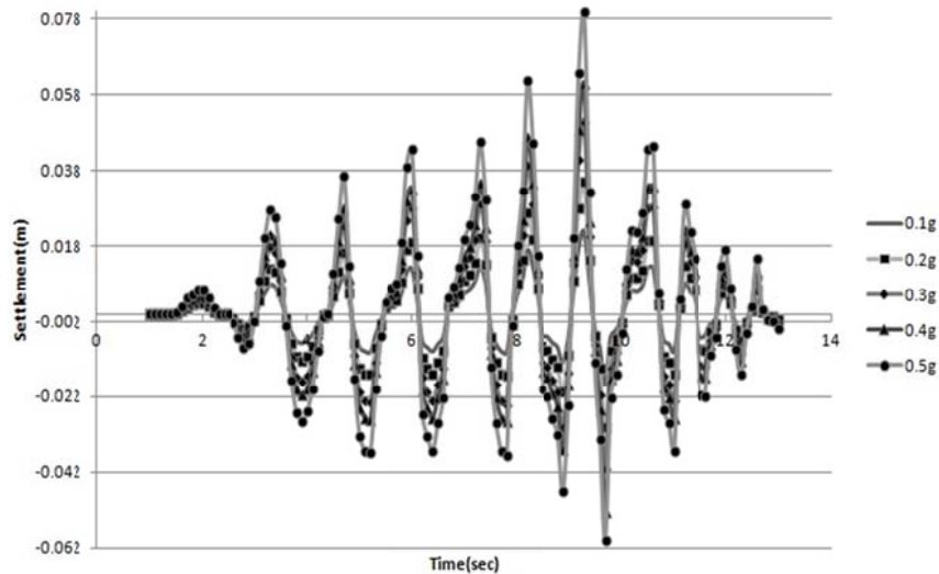
Fig. 7 Settlement and uplifting for unanchored tank in loose soil
