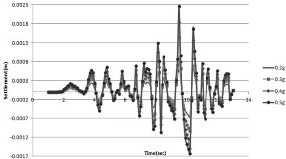
Fig. 4 Settlement and uplifting for anchored tank in dense soil
