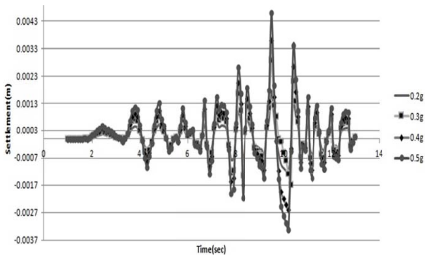
Fig. 6 Settlement and uplifting for anchored tank in medium soil
