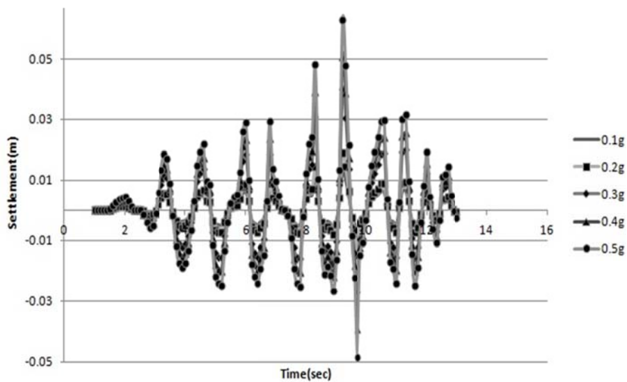
Fig. 5 Settlement and uplifting for unanchored tank in medium soil
