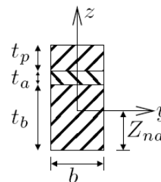
Fig. 1 A schematic of the cross section of the smart structure
