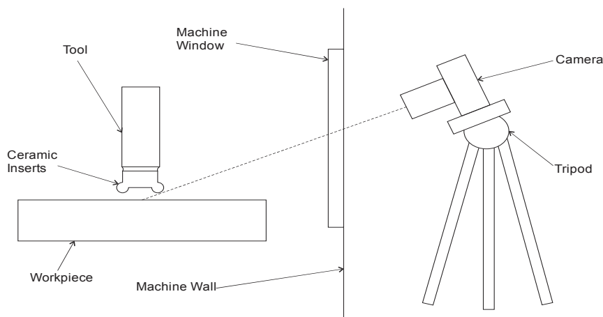
Fig. 2 Camera set-up
